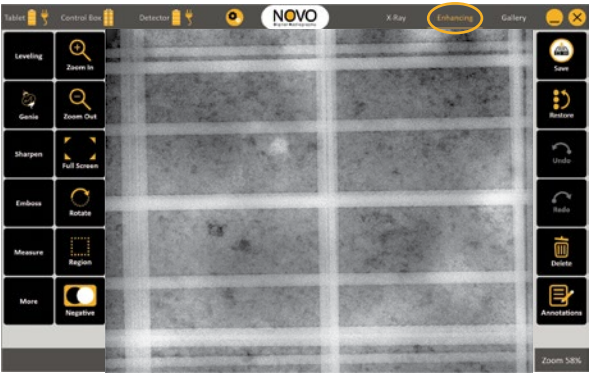
Enhancing Tab Rebars through a 6" ( 15.2cm) concrete wall Detector: NOVO 22WN Exposure time: 7s
